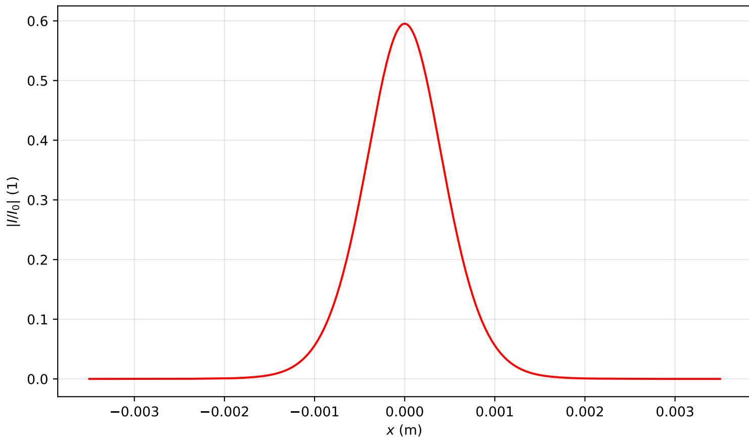
Intensity profile I(x, y = 0, z = 2.866)/I_0 , P_{in}=0.5P_{cr} , artificial time
